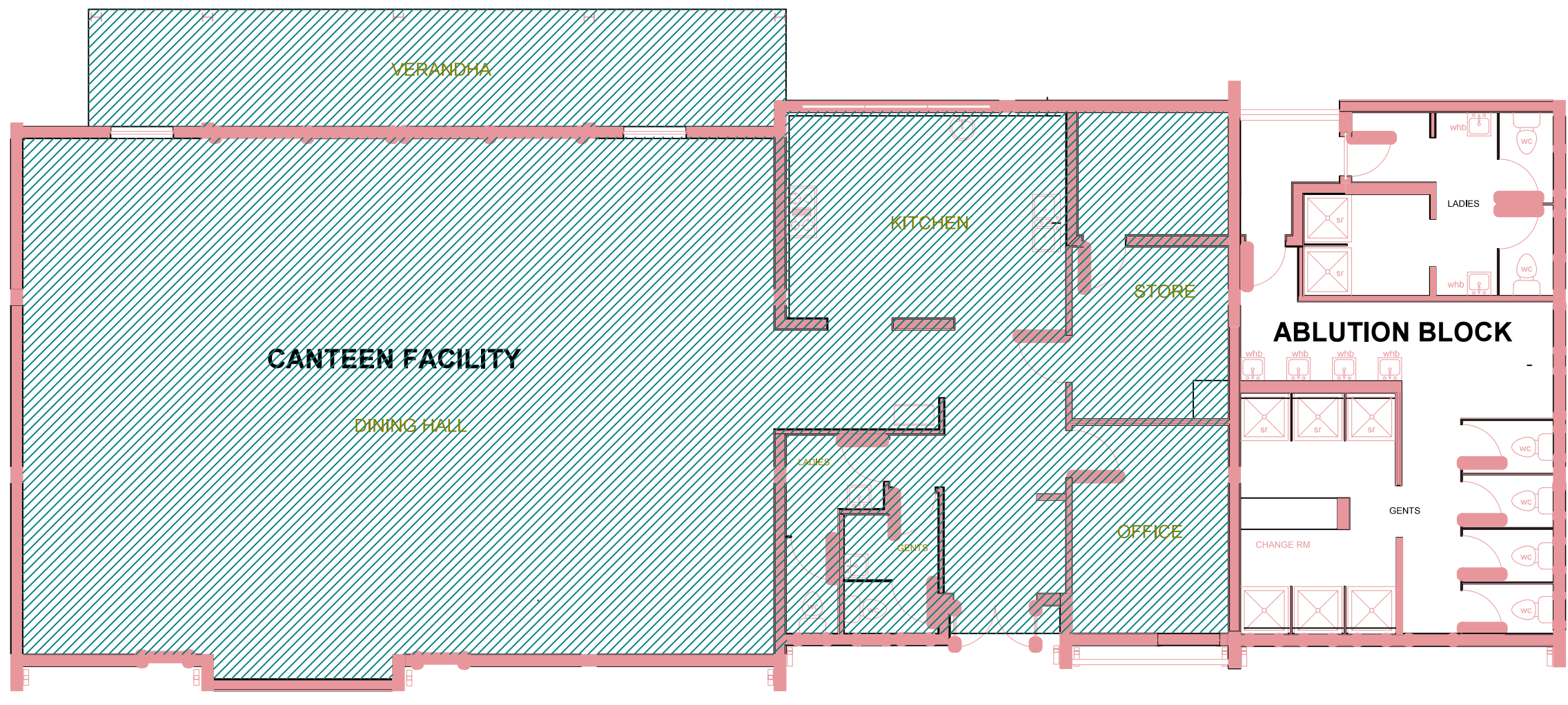
CANTEEN AND ABLUTION BLOCK LAYOUT
