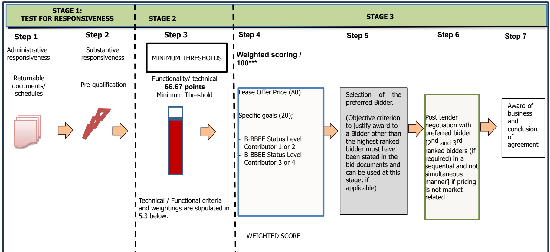
Diagram 1 Evaluation Methodology
