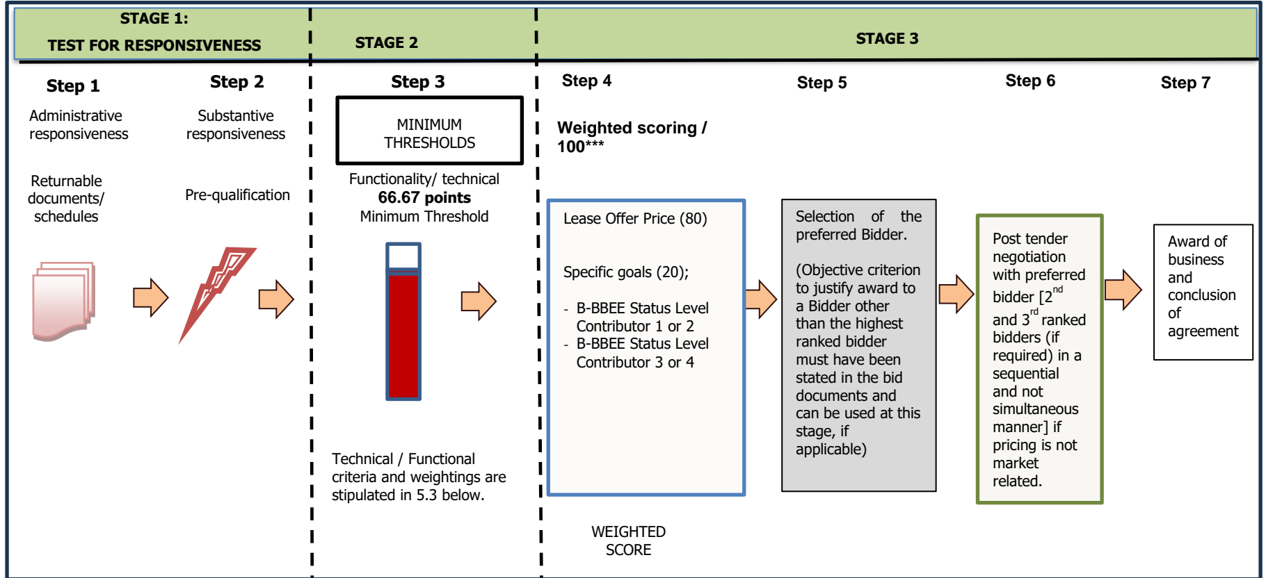
Diagram 1 Evaluation Methodology
