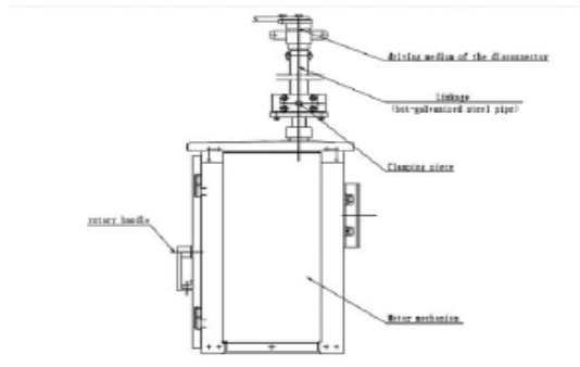
Drawing for installation of motor mechanism and disconnecter
