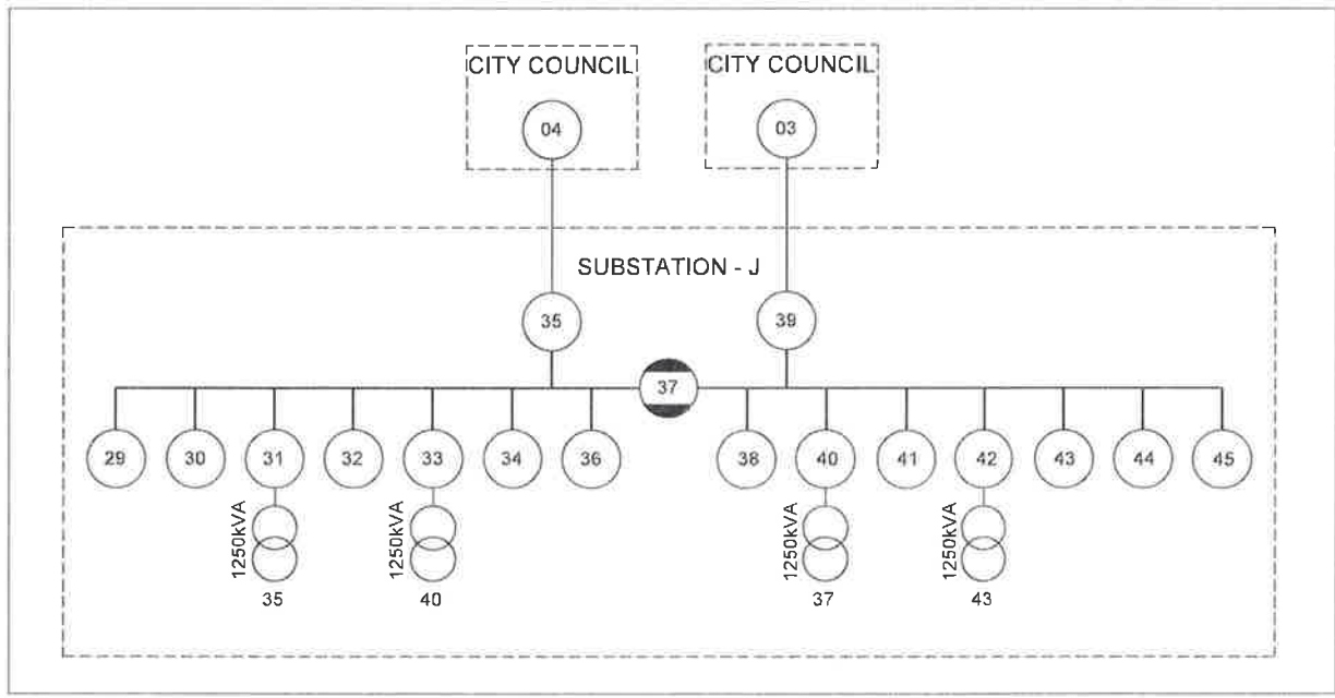
PROPOSED MEDIUM VOLTAGE SINGLE LINE DIAGRAM SCALE 1:100
