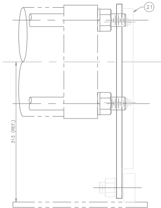
CYLINDER ROLLER ASSEMBLY
