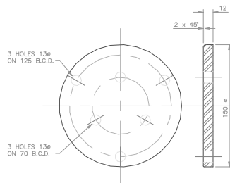
DETAIL - ITEM 9
