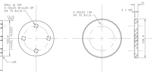
DETAIL - ITEM 11
