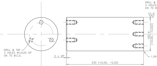
DETAIL - ITEM 10
